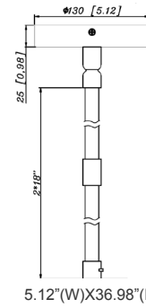
CMC2XL-MCT-DD-BK+CMC-SRK-218-5C-BK+CMC2-DCR-BG CMC2XL-MCT-DD-WH+CMC-SRK-218-5C-WH+CMC2-DCR-WG
