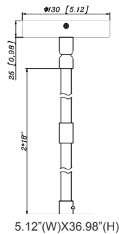
CMC2XL-MCT-DD-BK+CMC-SRK-218-5C-BK+CMC2-DS-BG CMC2XL-MCT-DD-WH+CMC-SRK-218-5C-WH+CMC2-DS-WG
