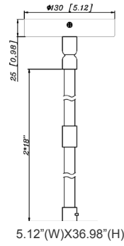
CMC2XL-MCT-DD-BK+CMC-SRK-218-5C-BK+CMC2-HCDK-AG CMC2XL-MCT-DD-WH+CMC-SRK-218-5C-WH+CMC2-HCDK-BK
