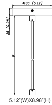
CMC2XL-MCT-DD-BK+CMC-CS-8FT-BK+CMC2-TRM-AG CMC2XL-MCT-DD-WH+CMC-CS-8FT-WH+CMC2-TRM-BN
